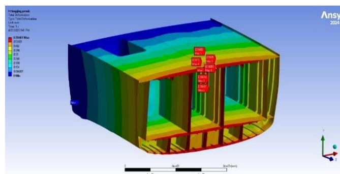
Figure 24. Results of Deflection conditions Hogging-full
