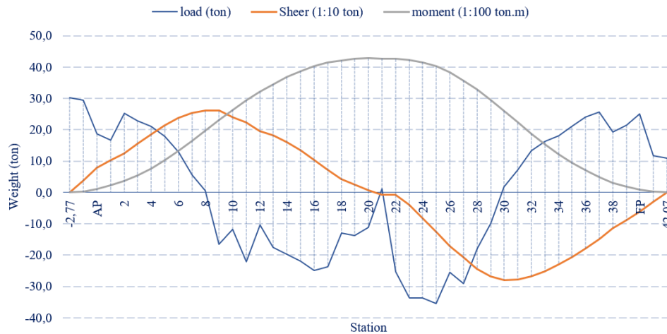
Figure 14. Full Condition Strength Chart Hogging
