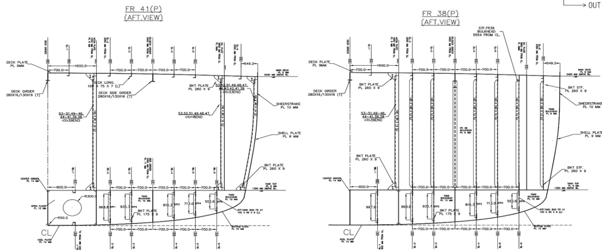
Figure 1. Construction Midship Ship
