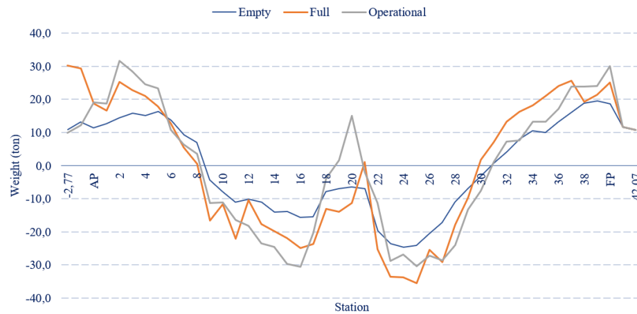
Figure 11. Condition Load Distribution Sagging
