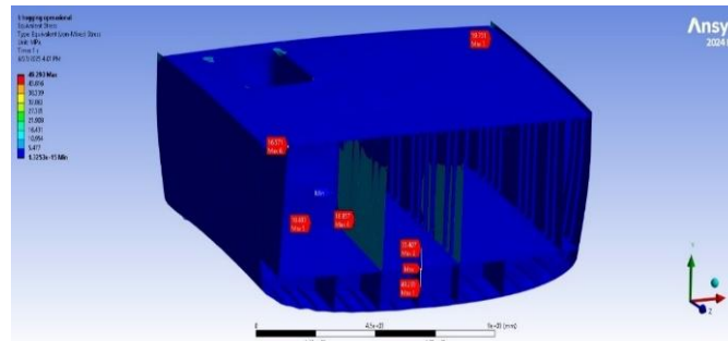
Figure 25. Result Stress condition Hogging-Operational
