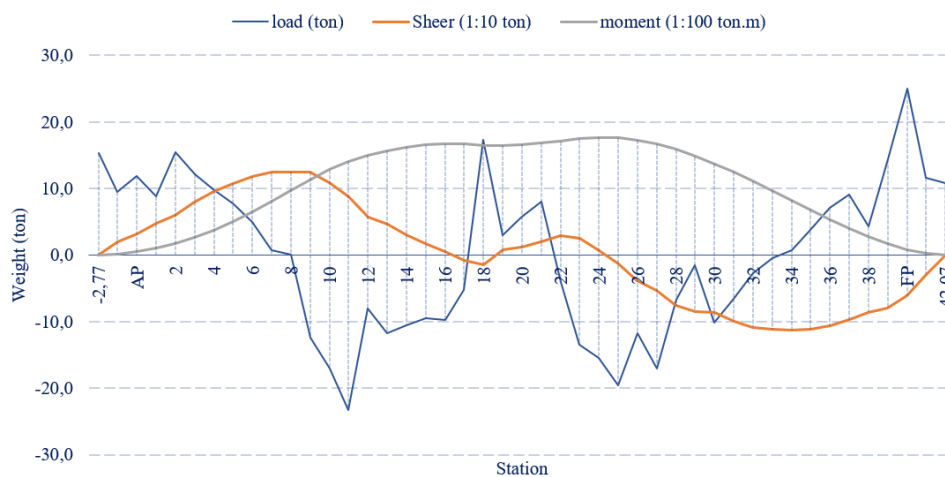
Figure 12. Full condition strength chart Sagging
