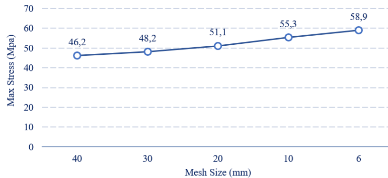
Figure 18. Mesh Convergence Test
