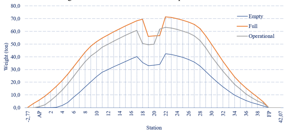
Figure 9. Distribution Buoyancy Conditions Hogging
