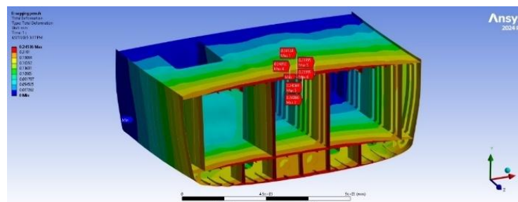
Figure 20. Results of Deflection conditions Sagging-full
