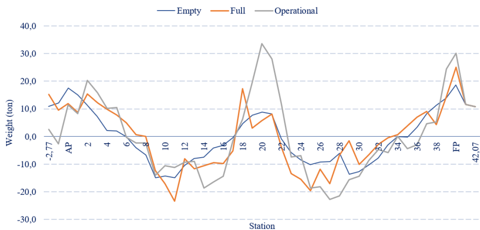
Figure 10. Condition Load Distribution Sagging
