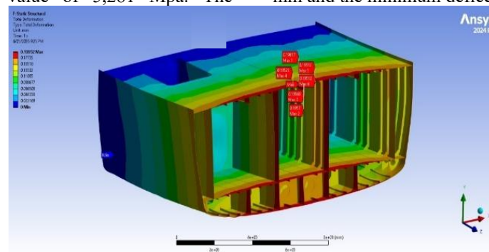
Figure 22. Results of Deflection conditions Sagging-Operational
