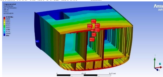
Figure 26. Results of Deflection conditions Hogging-Operational
