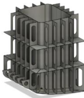
Figure 17. 3D model Moonpool Area
