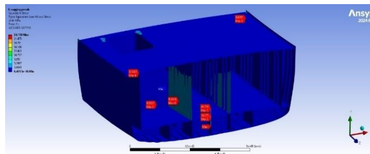
Figure 19. Result stress condition Sagging-full
