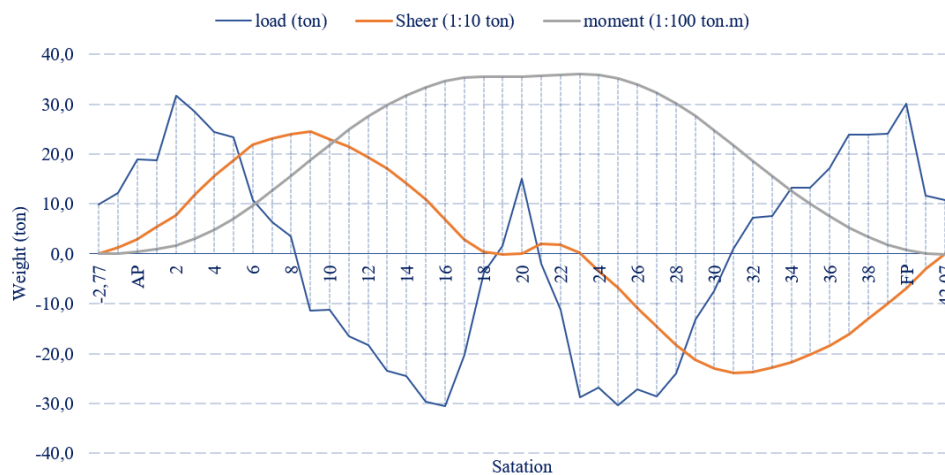
Figure 15. Graph of the strength of Operational conditions Hogging
