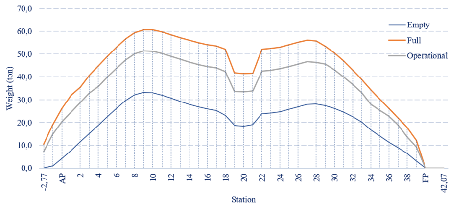
Figure 8. Distribution Buoyancy Conditions Sagging
