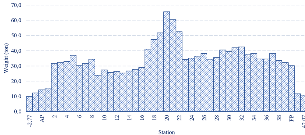
Figure 5. Heavy Distribution of Operational Cargo Vessels
