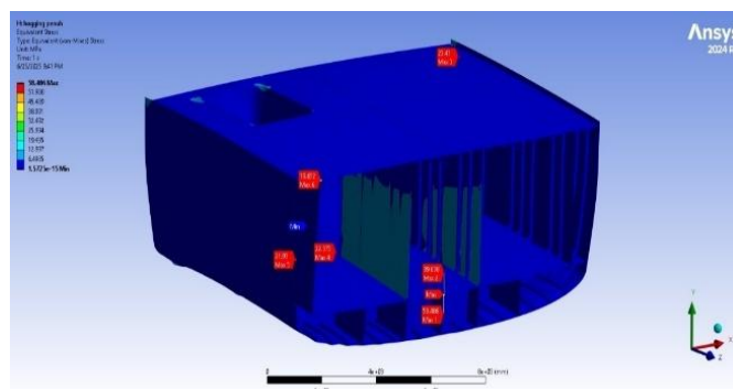
Figure 23. Result stress condition Hogging-Full
