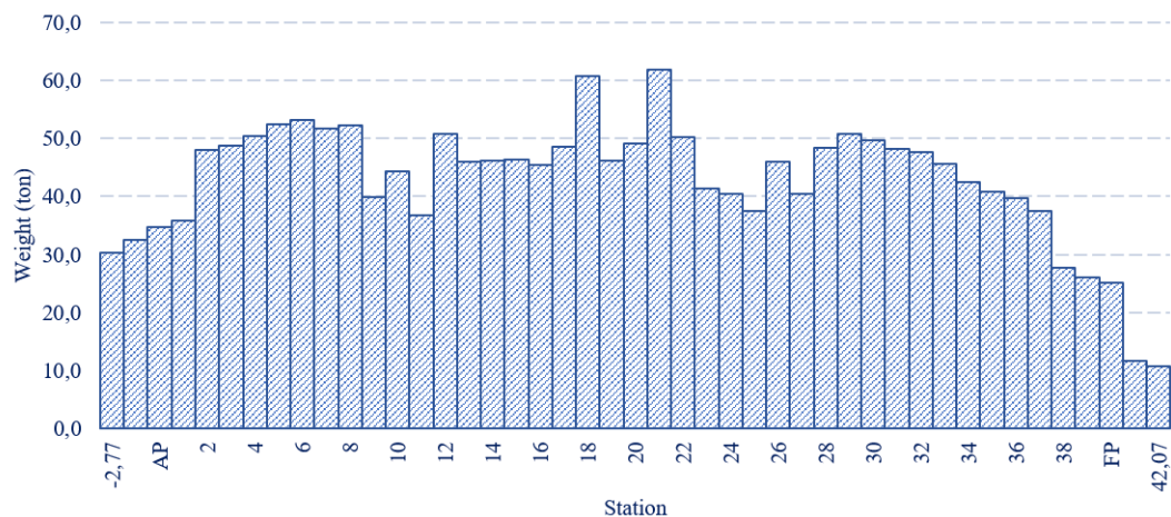
Figure 4. Distribution of Full Cargo Vessels
