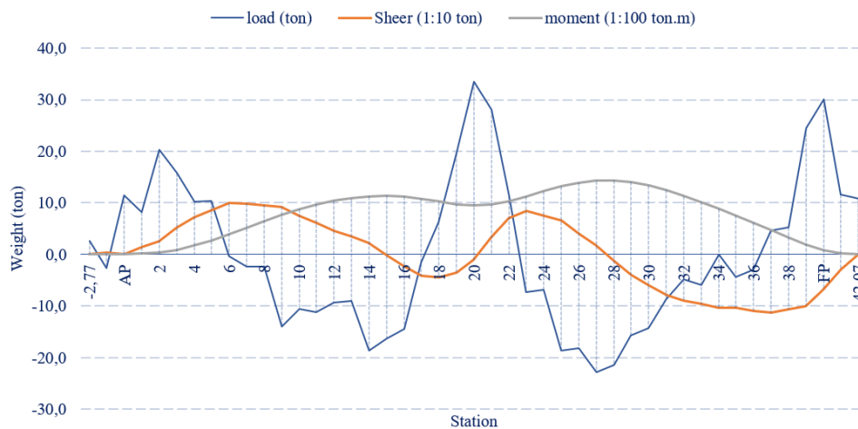
Figure 13. Graph of the strength of Operational conditions Sagging
