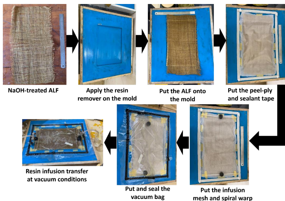
Figure 1. Fabrication of epoxy/ALF using resin infusion transfer method
