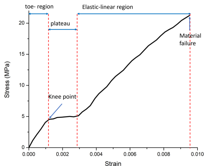
Figure 4. Example of stress – strain curve of epoxy/ALF composites
