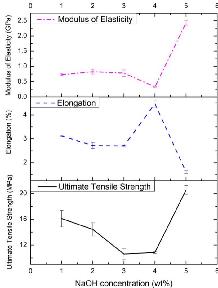
Figure 6. Modulus of elasticity, maximum elongation, and ultimate tensile stress of epoxy composite reinforced by ALF treated in various concentration of NaOH for 4 hours immersion
