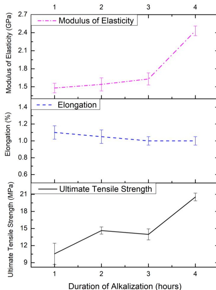
Figure 5. Modulus of elasticity, maximum elongation, and ultimate tensile stress of epoxy composite reinforced by ALF treated in NaOH 5 wt% for various durations
