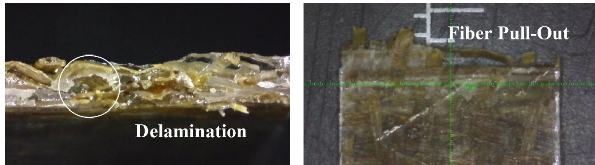
Figure 3. Section area (left) and fracture plane (right) of epoxy/ALF composites
