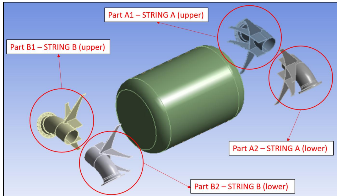
Figure 11. Extent for Local Structure Modeling of MWB
