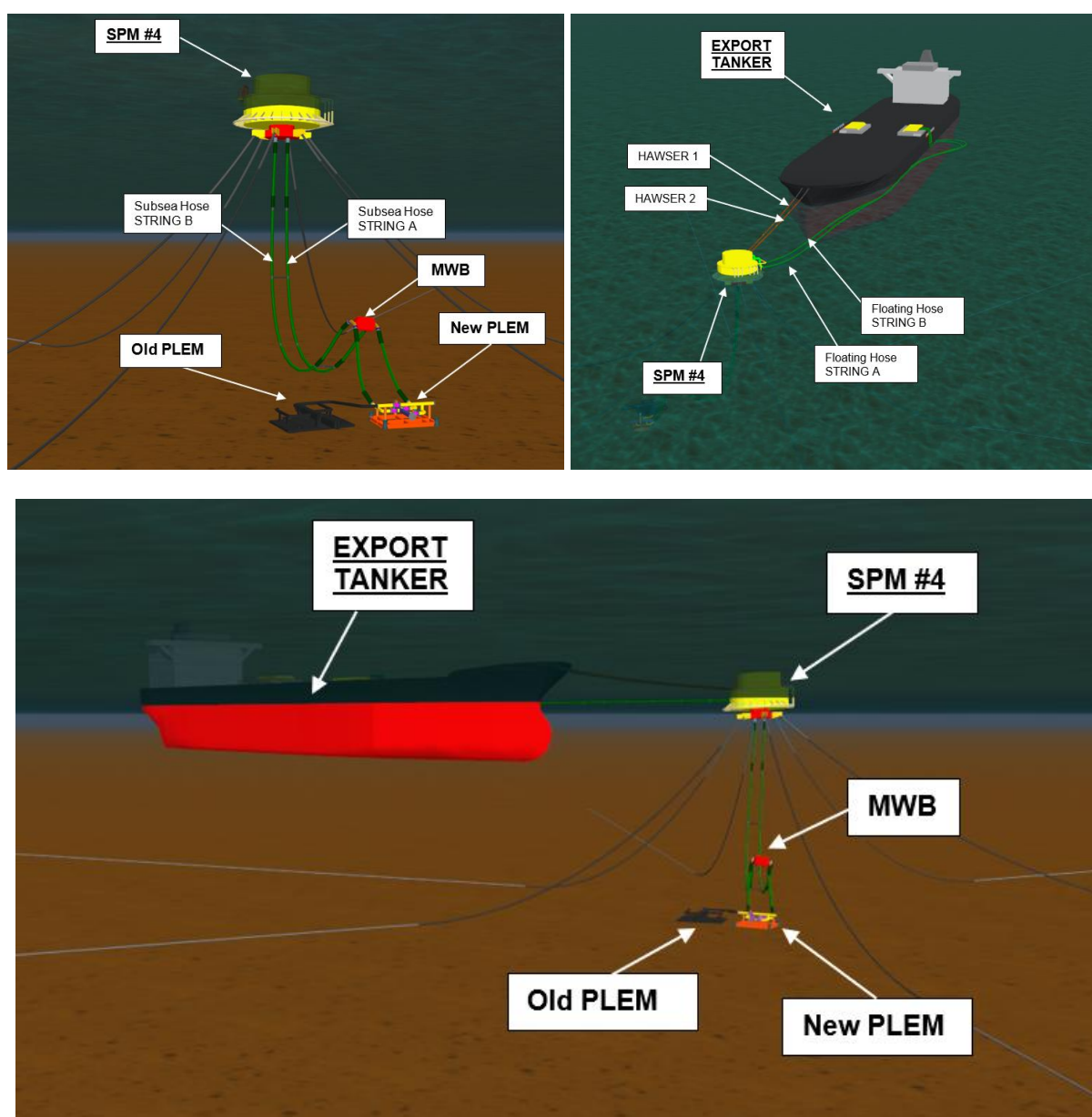
Figure. 6. Mooring System and Marine Hoses Modeling
