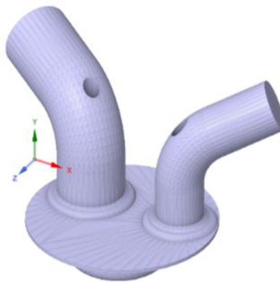
Figure 2. 3D Simulation Model
