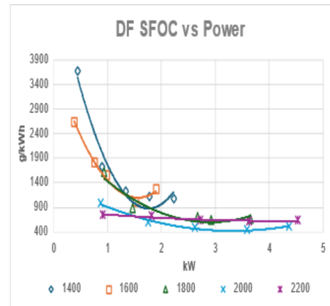
Figure 18. Specific fuel consumption of dual fuel NH 3 -B100
