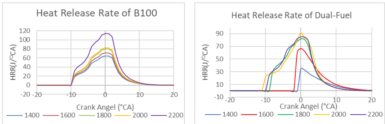
Figure 7. Heat Release Rate of B100 and NH 3 -B100
