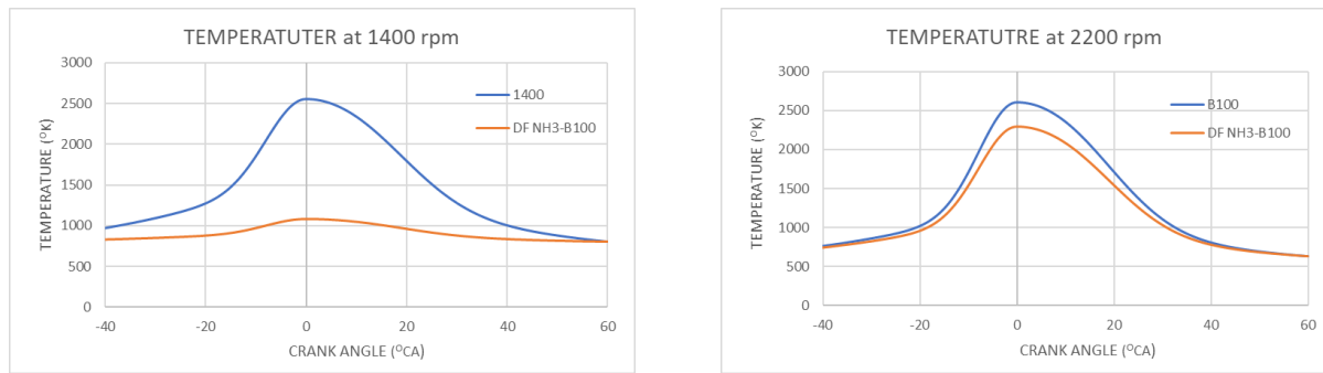
Figure 22 Difference In Temperature Trends Between B100 Single Fuel And NH3-B100 Dual Fuel At 1400 And 2200 Rpm
