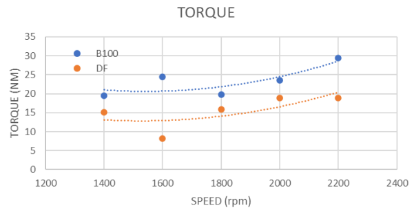
Figure 20. Comparison torque between B100 and dual fuel NH 3 -B100
