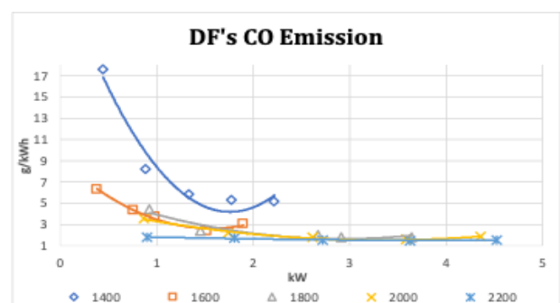
Figure 13. CO emission of dual fuel NH 3 -B100
