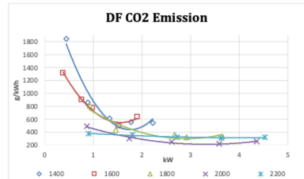
Figure 11. Dual Fuel CO2 Emission
