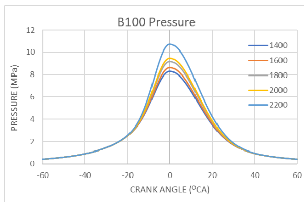
Figure 4. B100's Pressure vs Crank Angle Degree
