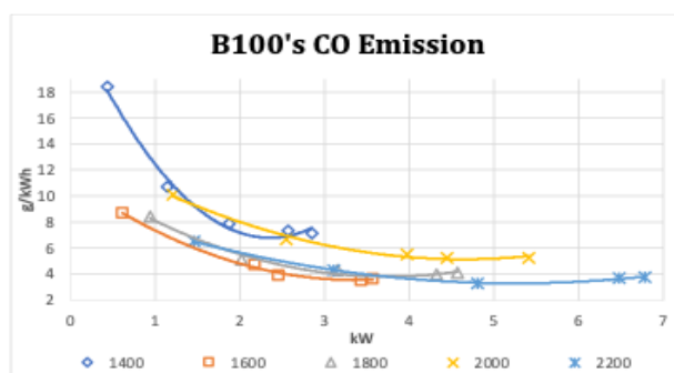
Figure 12. CO emission of B100
