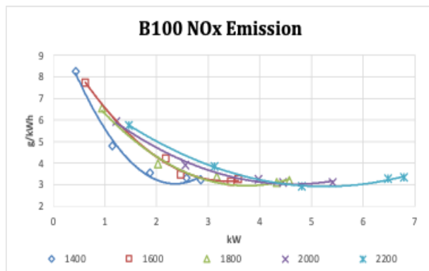
Figure 8. \text{NO}_x emission of B100
