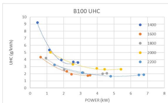
Figure 14 UHC emission of B100
