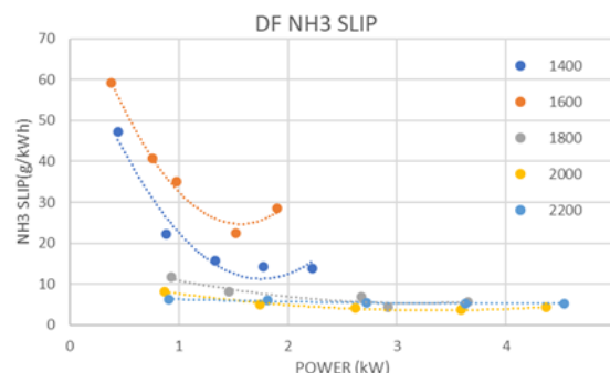
Figure 16. \text{NH}_3 Slip
