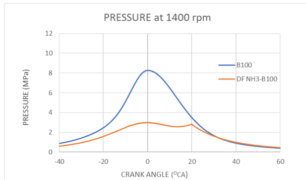
Figure 21 Difference In Pressure Trend Between Single Fuel B100 And Dual Fuel NH 3 -B100 At 1400 And 2200 Rpm
