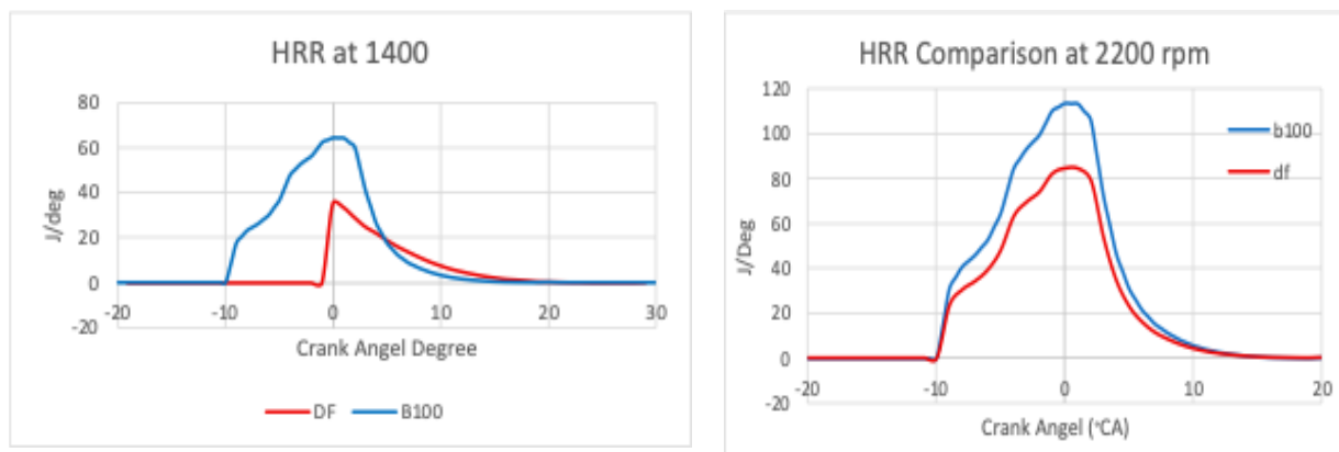
Figure 23. Difference In HRR Trends Between B100 Single Fuel And NH3-B100 Dual Fuel At 1400 And 2200 Rpm
