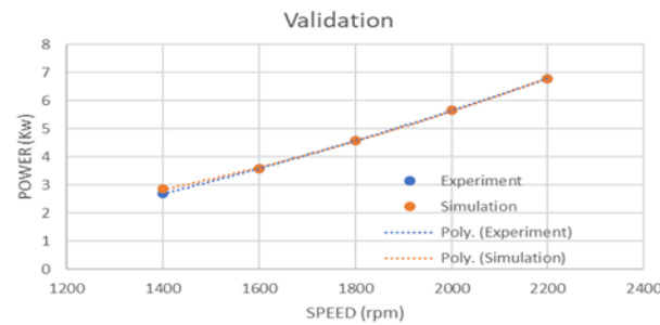
Figure 3. Comparison between Simulation and Experiment
