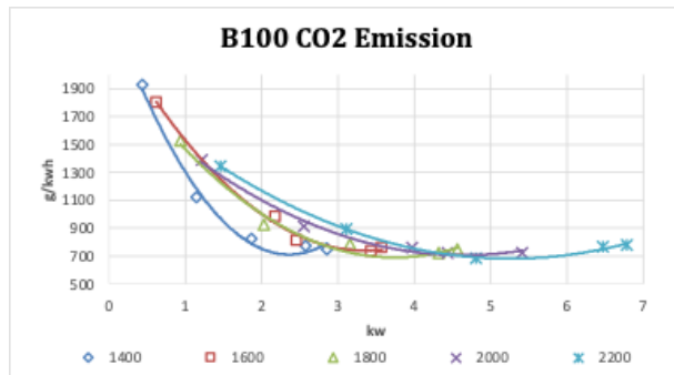
Figure 10. B100 CO2 Emission
