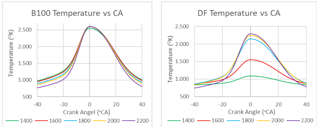
Figure 6. Temperature vs CA degree of B100 and Dual-Fuel (NH 3 -B100)
