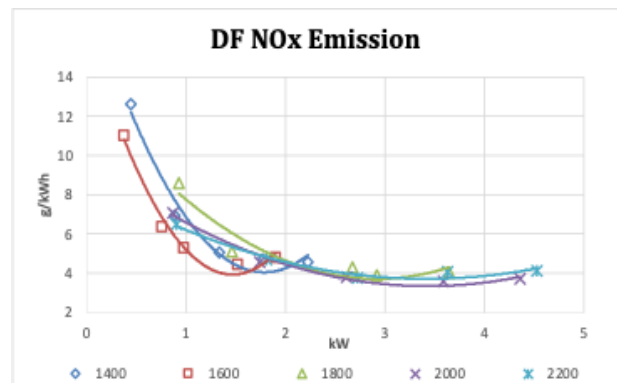
Figure 9. \text{NO}_x emission of dual fuels \text{NH}_3 -B100
