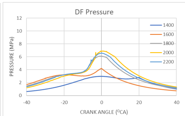
Figure 5. Dual-Fuel's Pressure vs Crank Angle Degree
