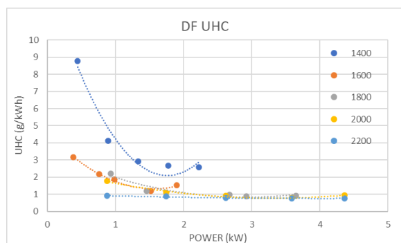
Figure 15. UHC emission dual fuel of \text{NH}_3 –B100
