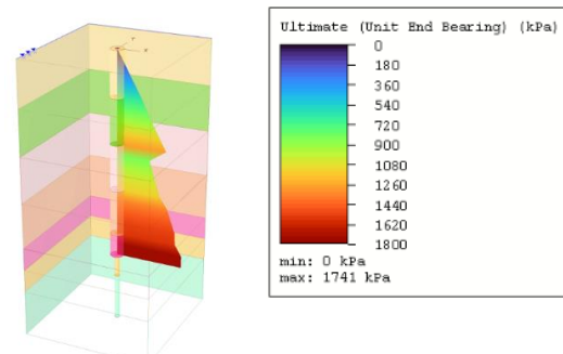
Gambar 6. Nilai f_b hasil analisis RS Pile.
