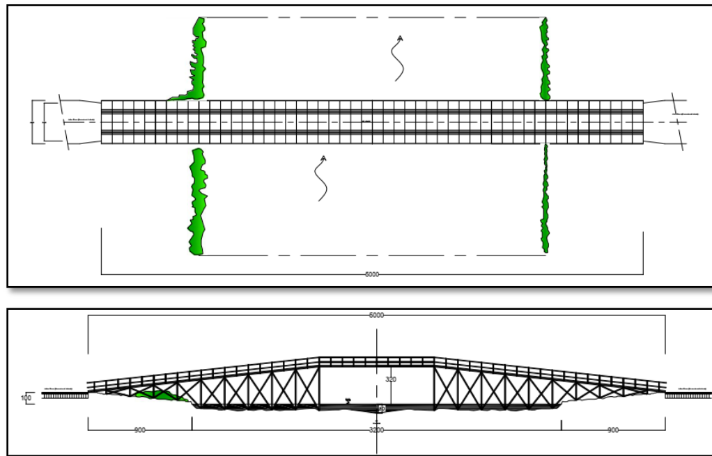
Figure 3. Top View and Longitudinal View Muara Tahai Bridge, Sta. 0+100
