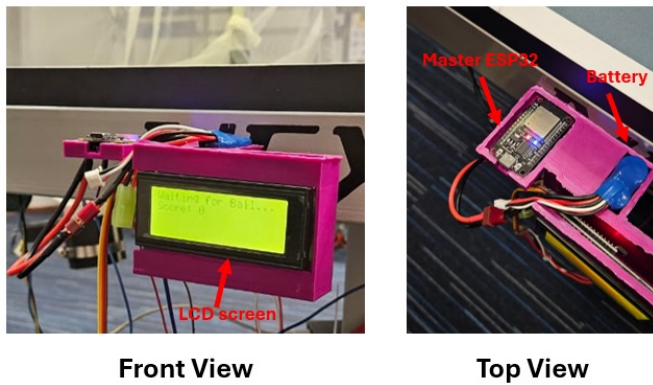
Figure 4. Master ESP32.
