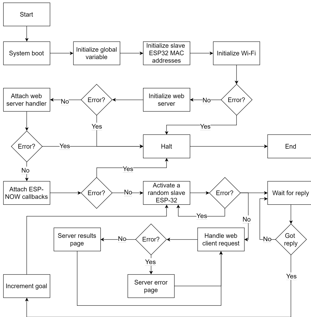
Figure 6. Flow diagram of a master ESP32 program.
