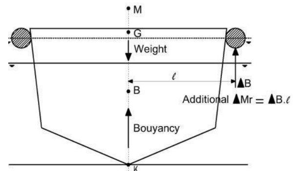
Figure 2. Contribution of side floater
