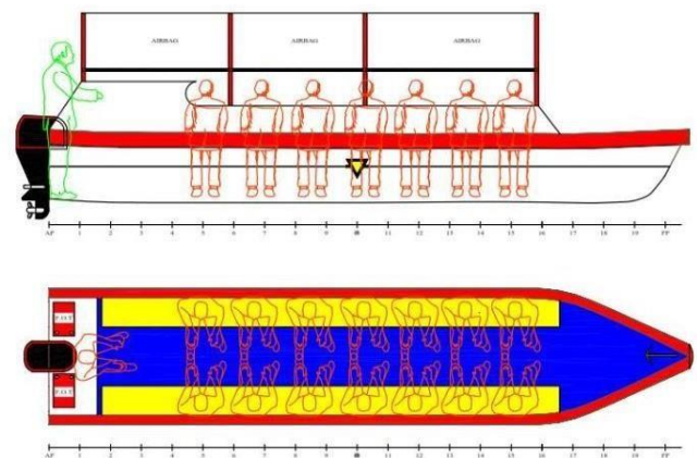
Figure 4. The general arrangement of boat
