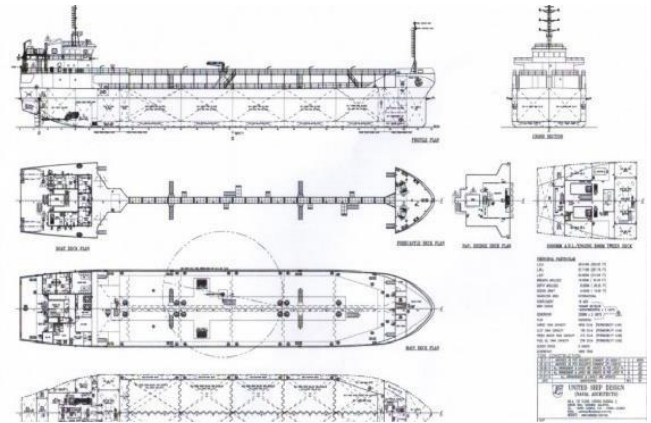
Figure 2. General Arrangement of Oil Tanker 4999 DWT
