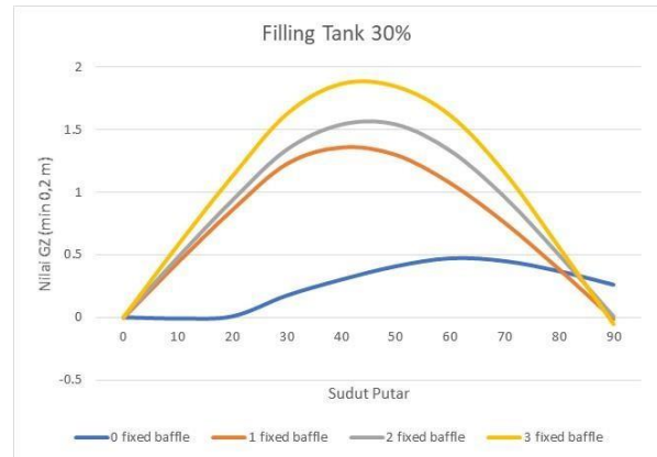
Figure 8. Graph of GZ value for condition I
