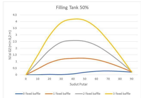
Figure 9. Graph of GZ Value at Condition II
