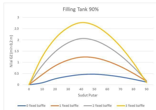
Figure 11. Graph of GZ Value at Condition I
