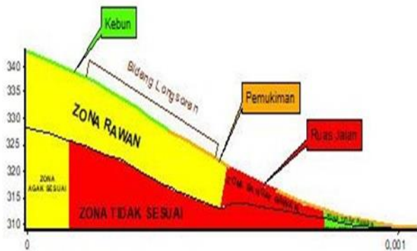
Figure 7. Results of Landslide Cross Section of Cikuya Village
