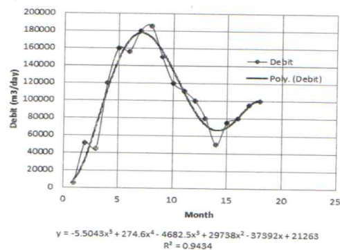
Fig. 4. The curve of mud blow out debit as recorded monthly
