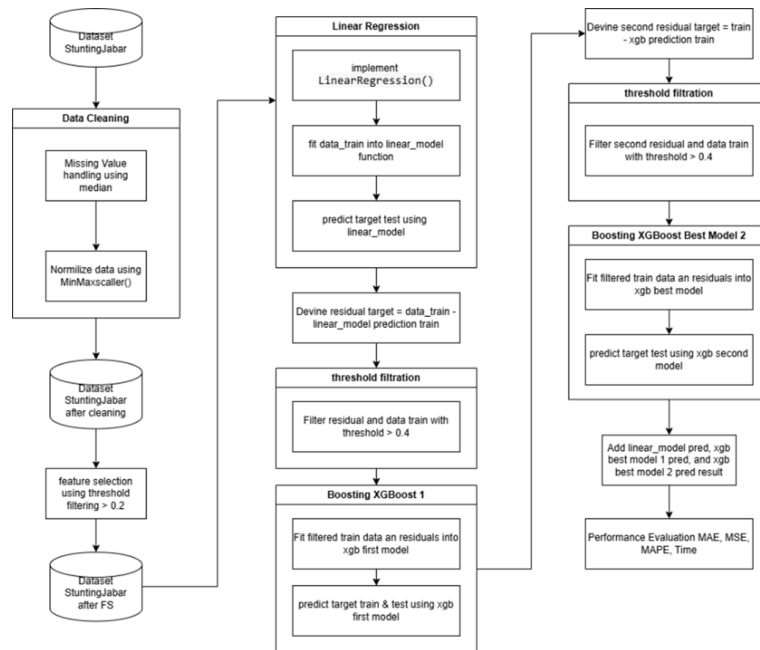
FIGURE 13 LR-XGB2 Modeling Flow
