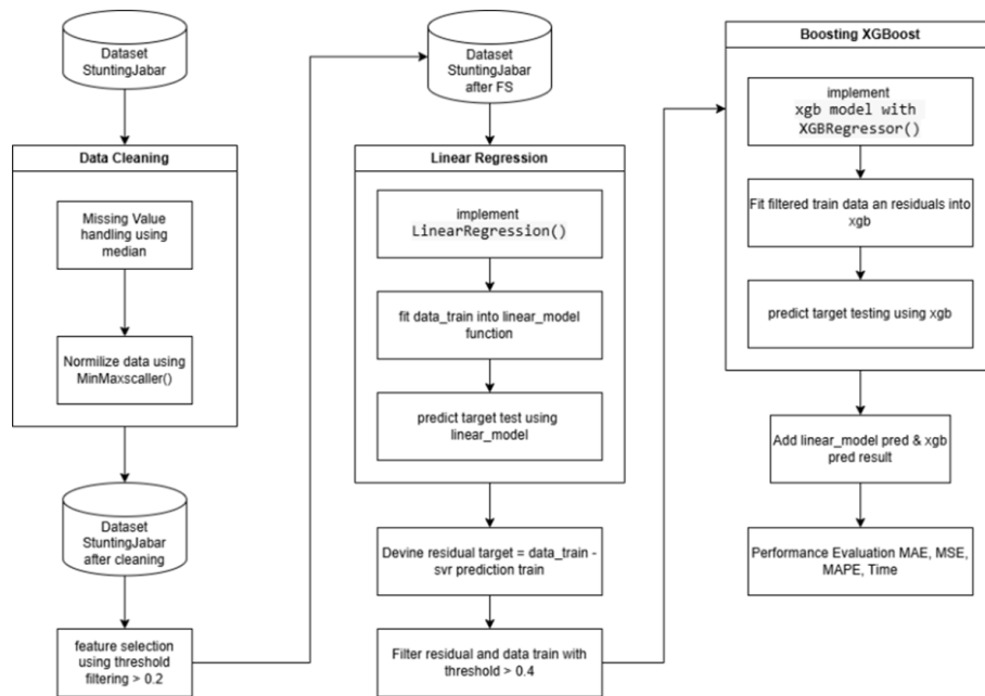
FIGURE 12 LR-XGB Modeling Flow
