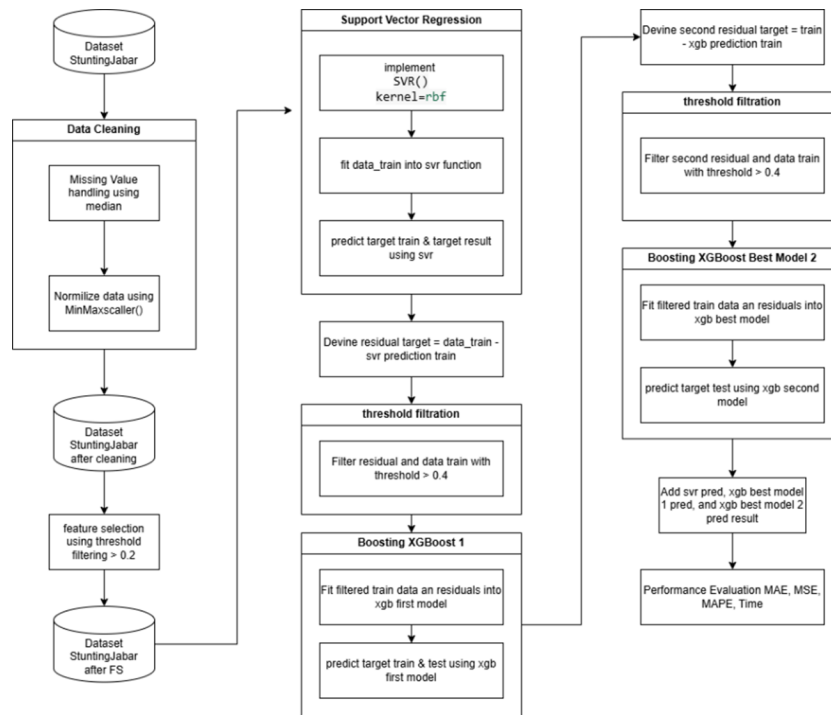
FIGURE 9 SVR-XGB2 Modeling Flow
