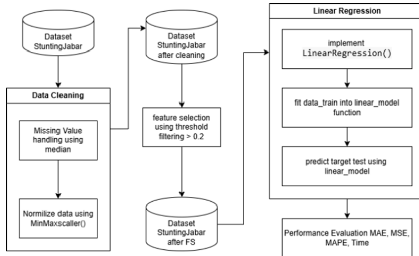
FIGURE 11 LR Modeling Flow
