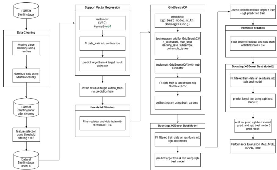
FIGURE 10 SVR-XGB2-Opt Modeling Flow
