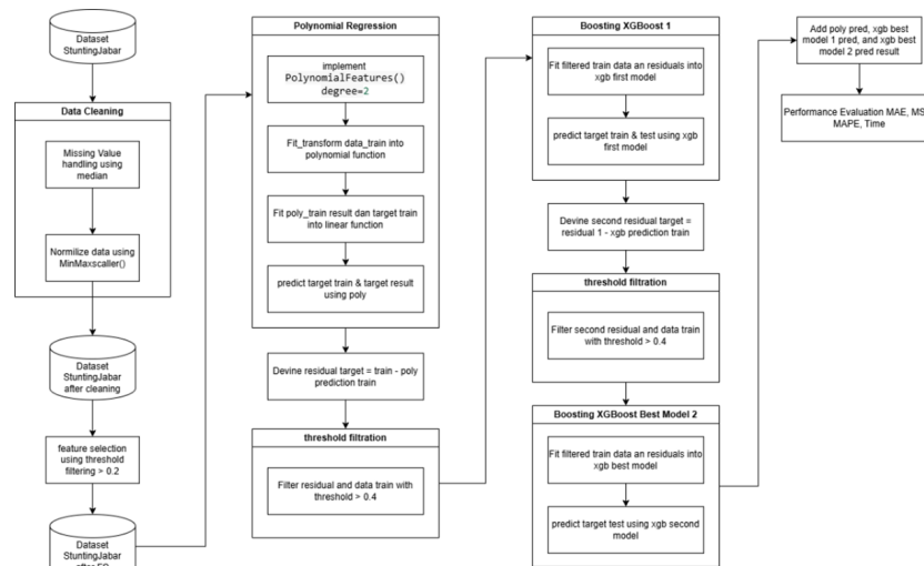
FIGURE 5 PR-XGB2 Modeling Flow
