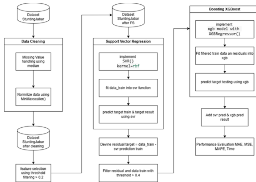
FIGURE 8 SVR-XGB Modeling Flow
