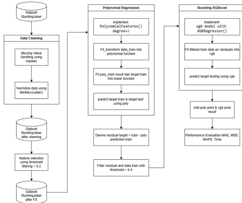
FIGURE 4 PR-XGB Modeling Flow
