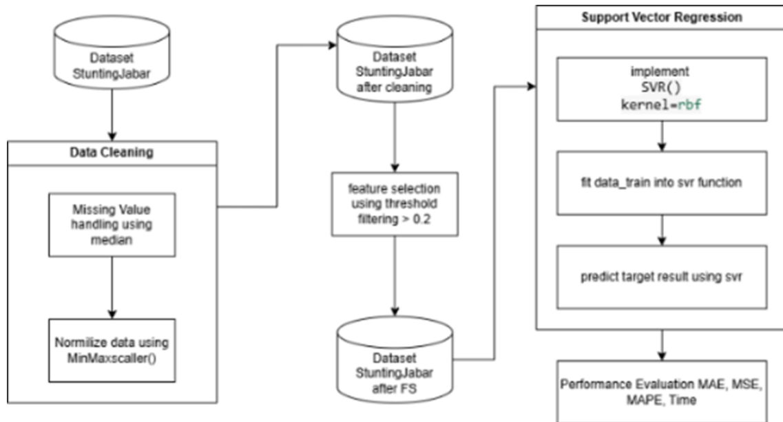
FIGURE 7 SVR Modeling Flow
