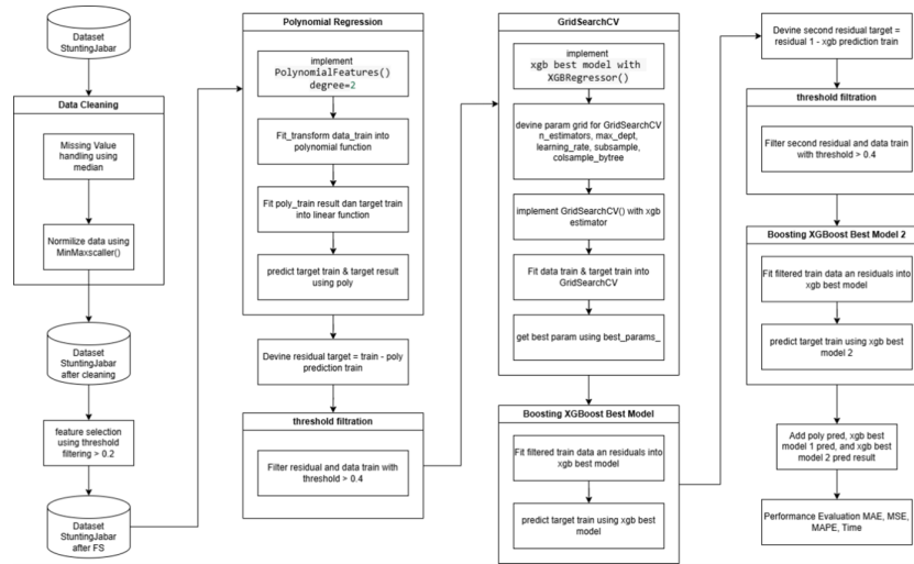
FIGURE 6 PR-XGB2-Opt Modeling Flow
