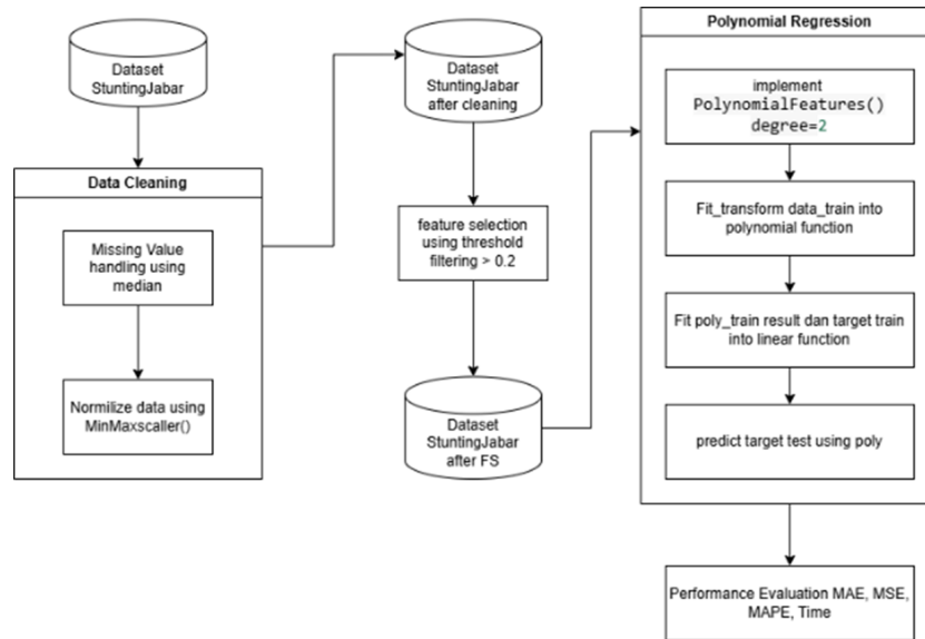
FIGURE 3 Polynomial Regression Modeling Flow
