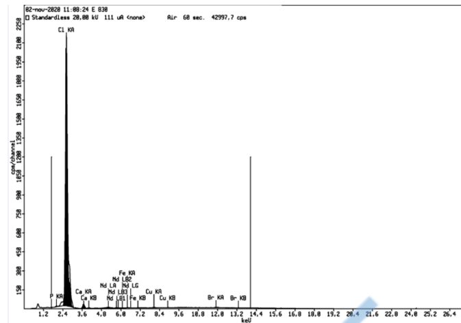
Gambar 4 Hasil uji XRF-standard sampel garam tambak.
