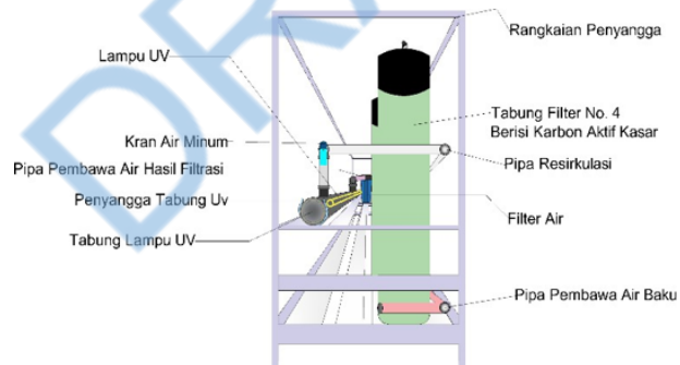
Gambar 6 Desain Filter Air.
